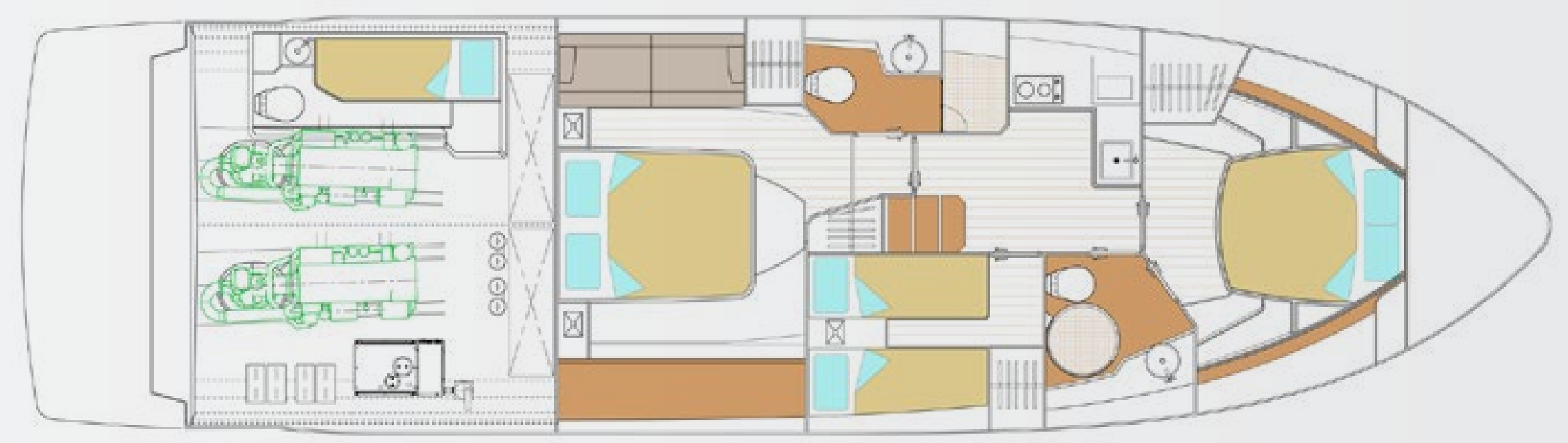
CABINS - OPTION 3
